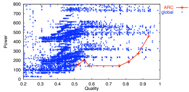
Figure 8. Global vs. ARC operation space.
