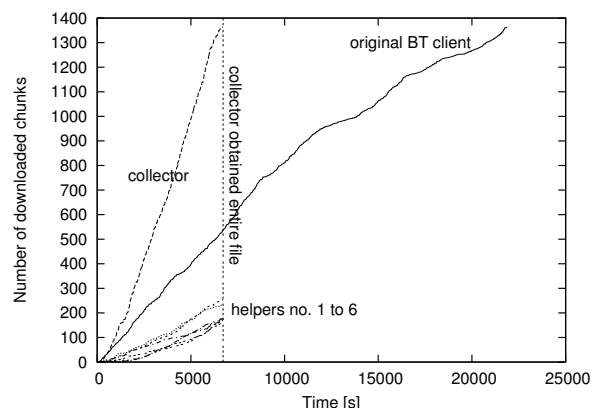
Figure 3. The download progress of a collector, its helpers and a BitTorrent peer.
