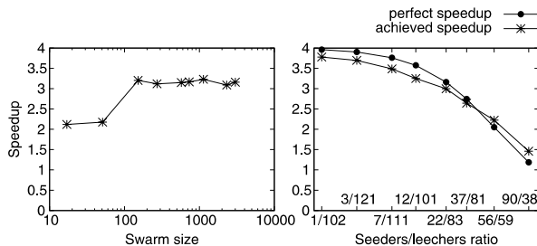
Figure 5. The influence of the swarm size on the speedup (left), and the influence of the seeders-to-leechers ratio on the speedup (right).
