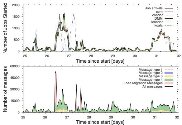
Fig. 6. System operation over time: ( top ) comparison of the number of jobs started by five grid resource management architectures. ( bottom ) the number of messages for DMM, per message type.
