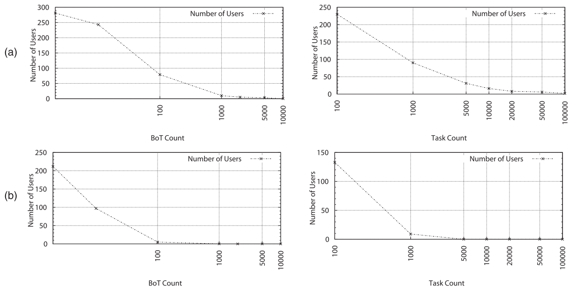
Fig. 1. Number of MTC users for the DAS-2 trace (a), and the San Diego Supercomputer Center (SDSC) SP2 trace (b) when considering only the submitted BoT count criterion ( left ), and only submitted task count criterion ( right ).
