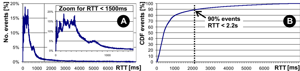
Fig. 3. The distribution of measured RTT: (a) detailed distribution and zoom to RTTs below 1.5 seconds; (b) CDF of RTT. The vertical axis shows the respective percentages of numbers of RTTs.
