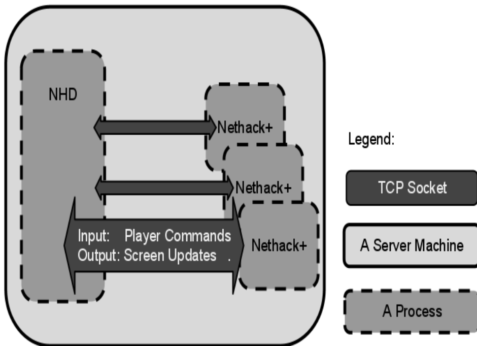
Figure 3.1: Schematic overview of a NHD with several Nethack+ processes.
