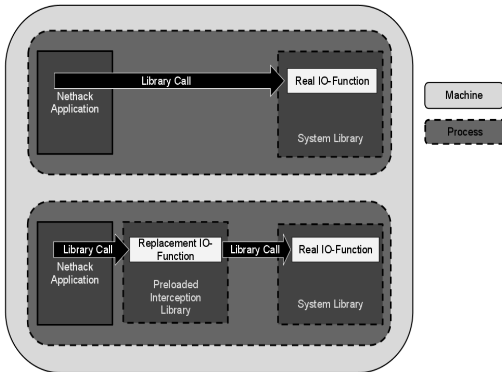
Figure 3.3: Example of library preloading.
